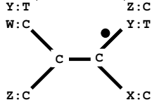
Tree 3: ((WZ)(XY))
