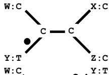
Tree 2: ((WY)(XZ))
