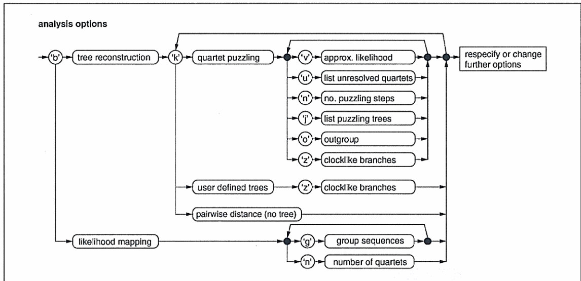
Figure 6.6.2 Flowchart of analysis type options in the TREE-PUZZLE menu. Options in TREE-PUZZLE are controlled by single letters. The flow chart shows the options that correspond to each letter. For example, entering the letter b toggles the analysis between tree reconstruction and likelihood mapping. Similarly, to choose among quartet puzzling, user-defined trees, or pairwise distance matrices, enter the letter k until the desired option is shown on the screen.
