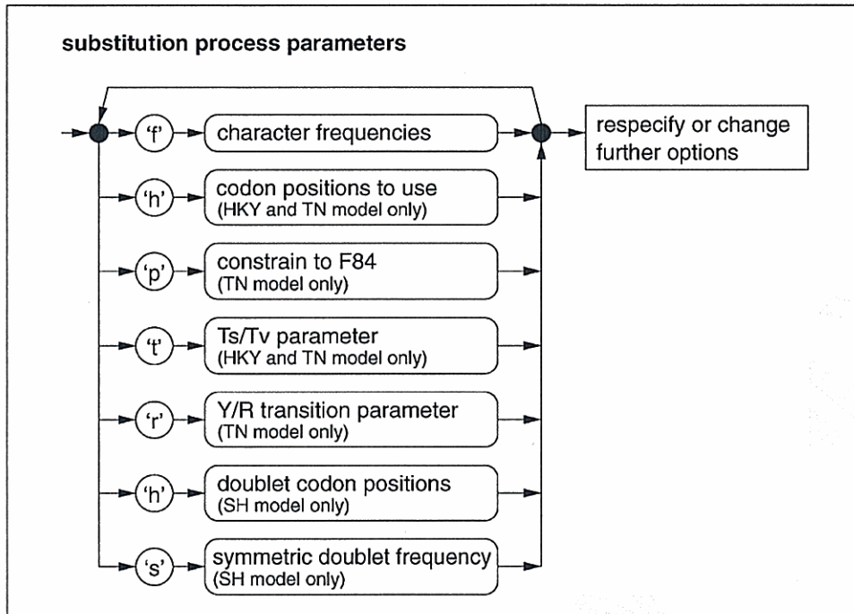
Figure 6.6.4 Flowchart of further substitution model parameters in the TREE-PUZZLE menu.
