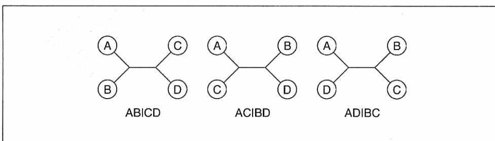
Figure 6.6.1 The three possible informative quartet tree topologies.
