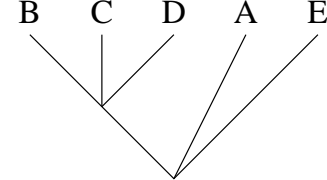
Adams consensus
