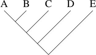
Tree A
