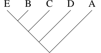
Tree B
