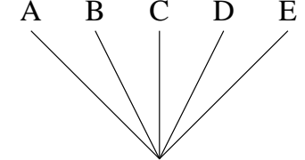
strict/majority consensus
